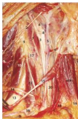
Fig. 7.7 Prescalene plane
